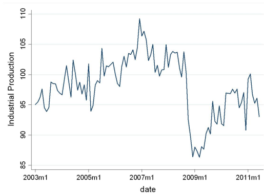
Figure 8: Industrial production
