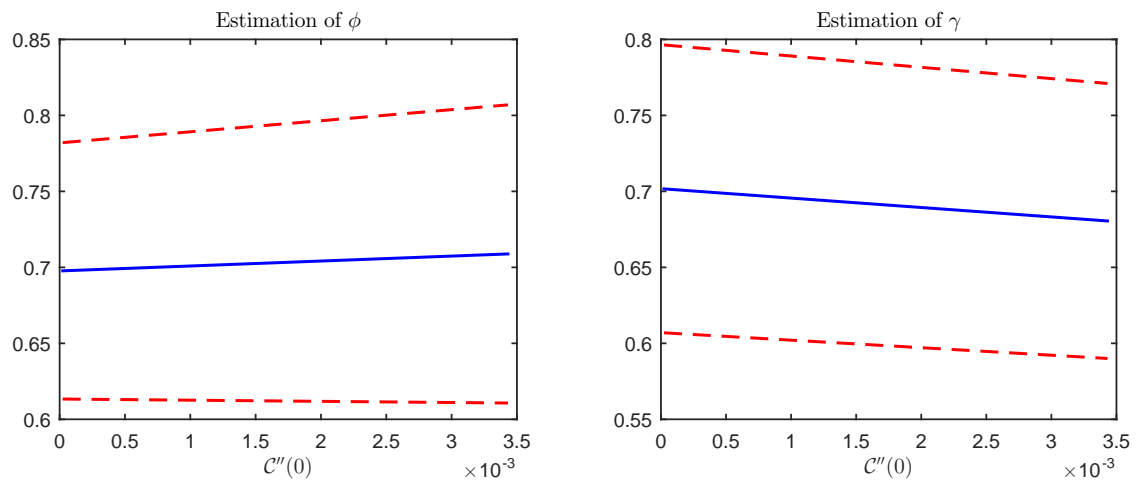
Figure 4: Estimation Results for Different Values of \mathcal{C}''(0)
